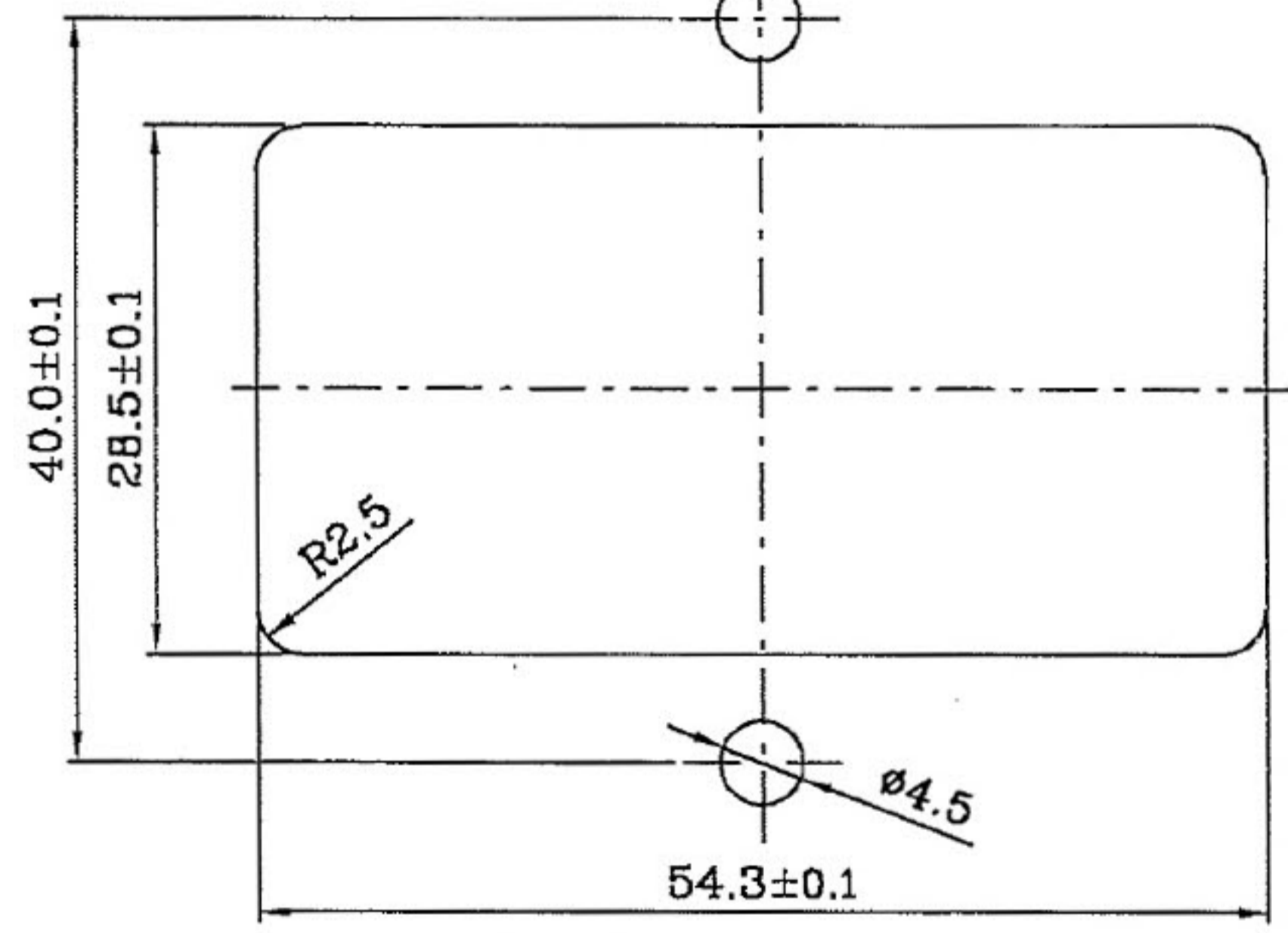
PANEL CUT-OUT
